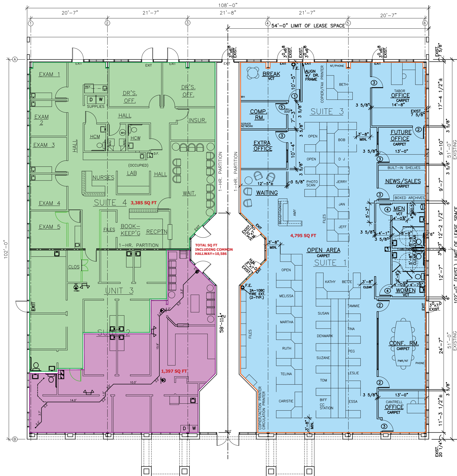
FLOOR PLAN – INTERIOR BUILD-OUT 1/8" = 1'-0"
