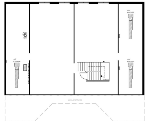
SECOND FLOOR STORAGE AREA
