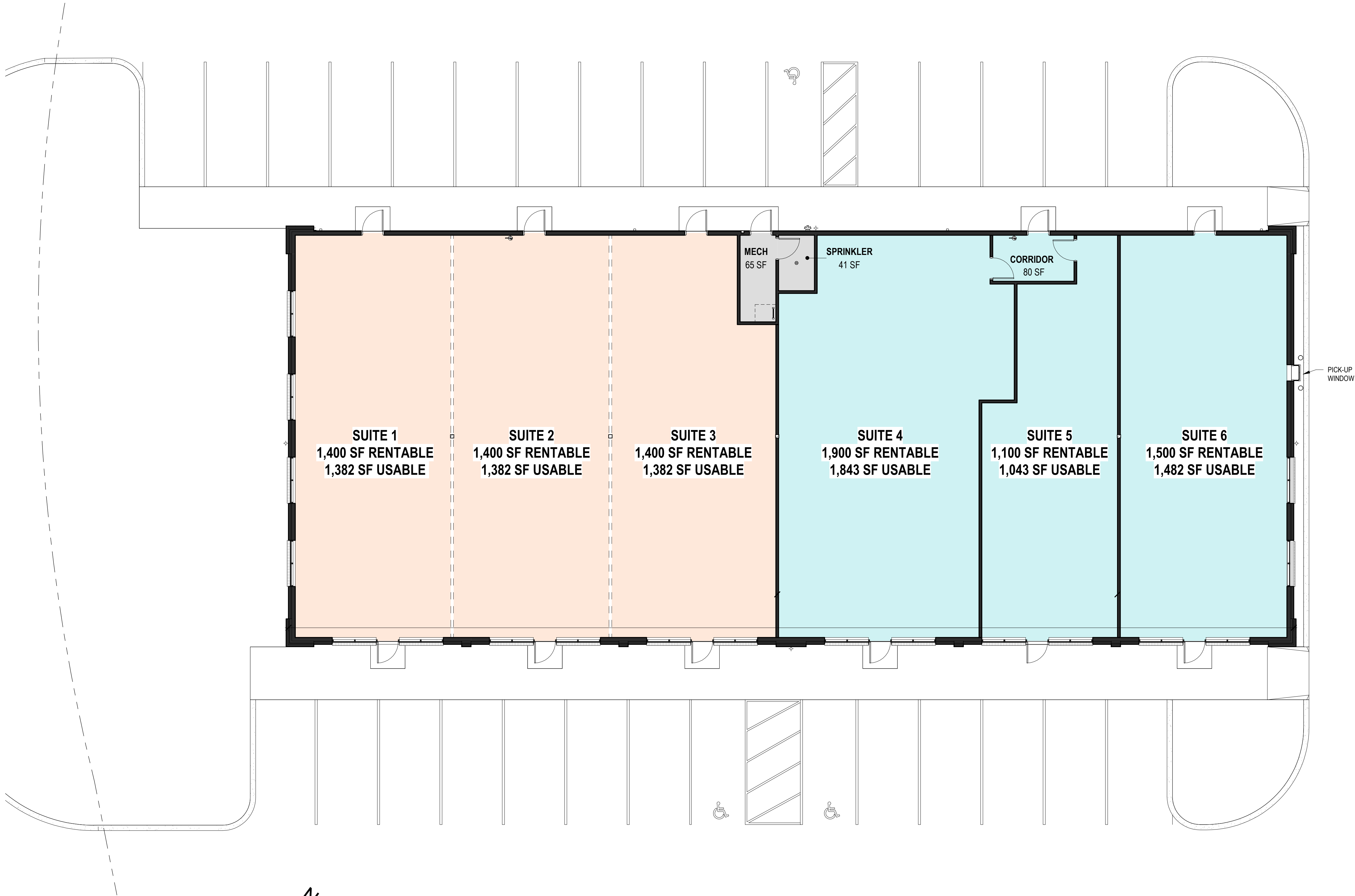
LEVEL ONE FLOOR PLAN 1/8" = 1'-0"
