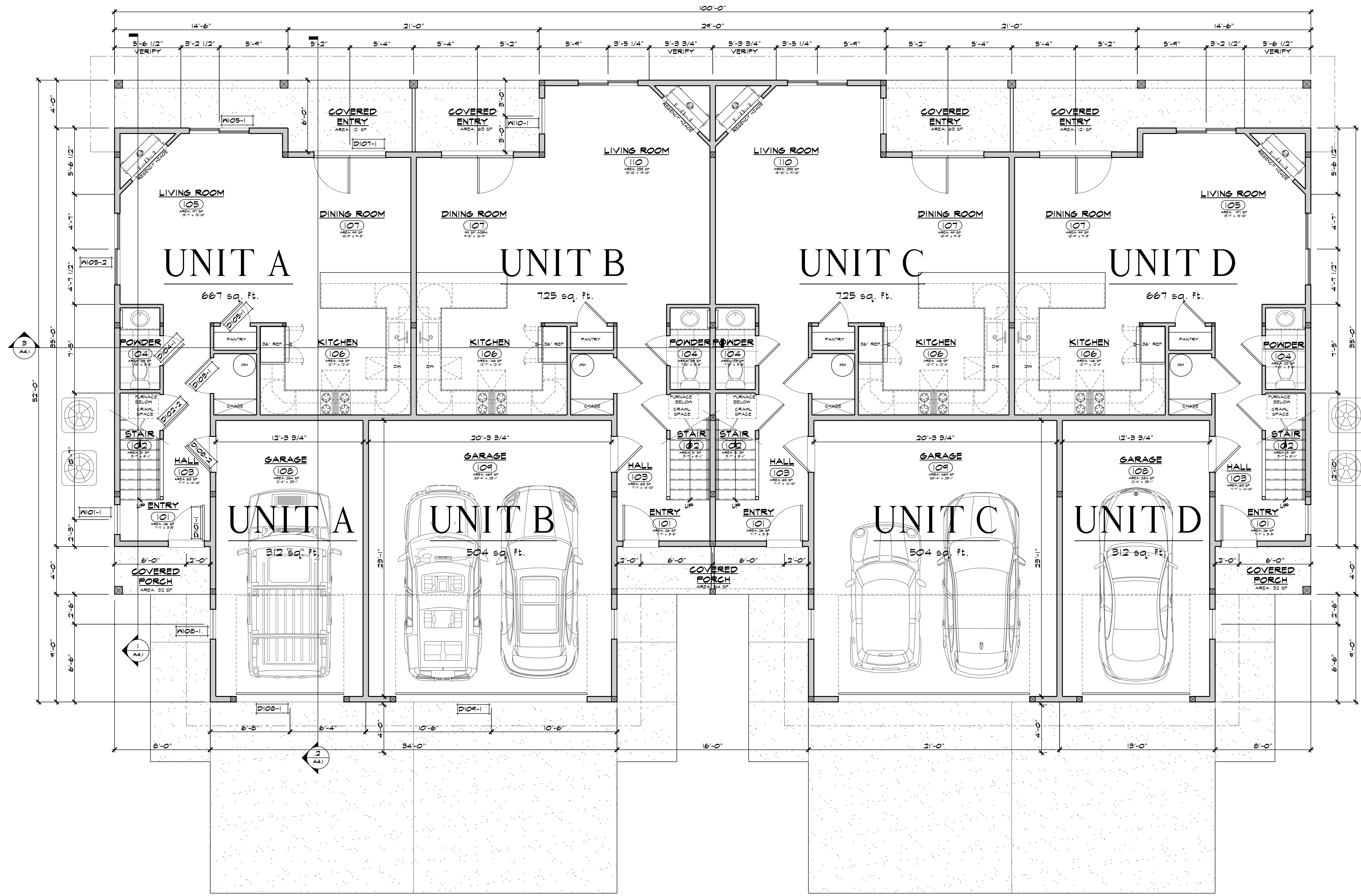
1 MAIN LEVEL FLOOR PLAN A2.1 SCALE: 1/4" = 1'-0"
