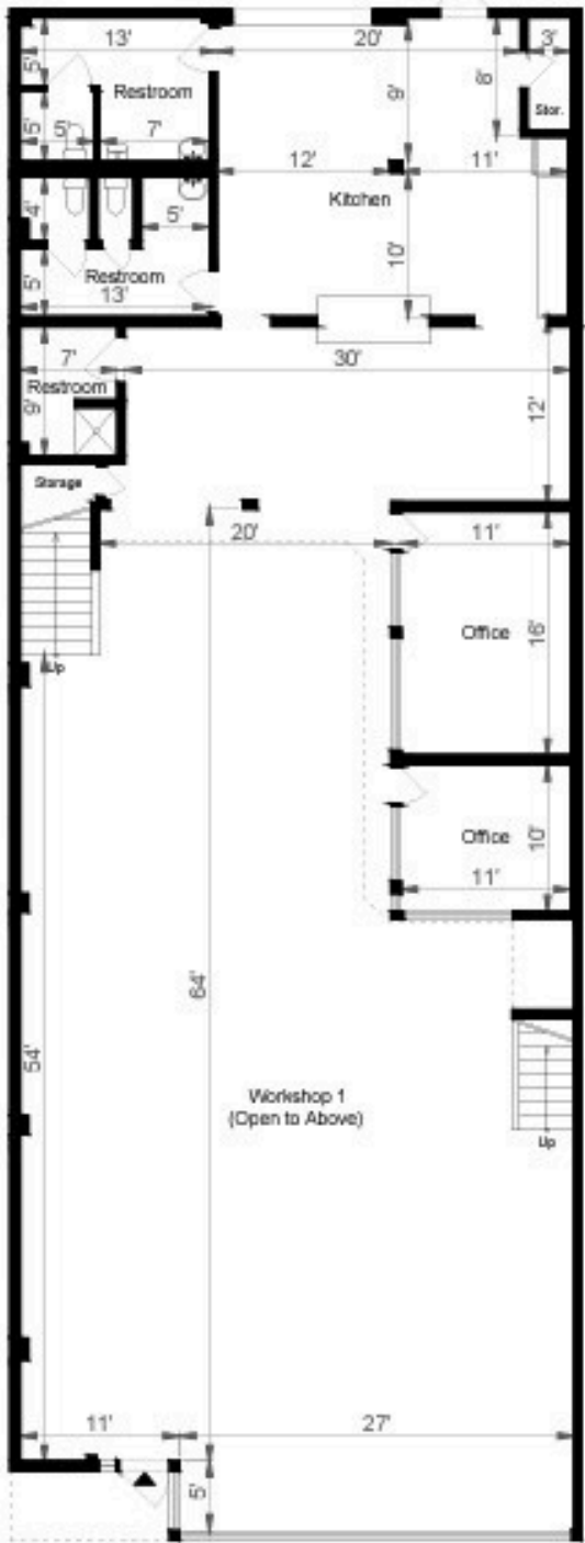
FIRST FLOOR
