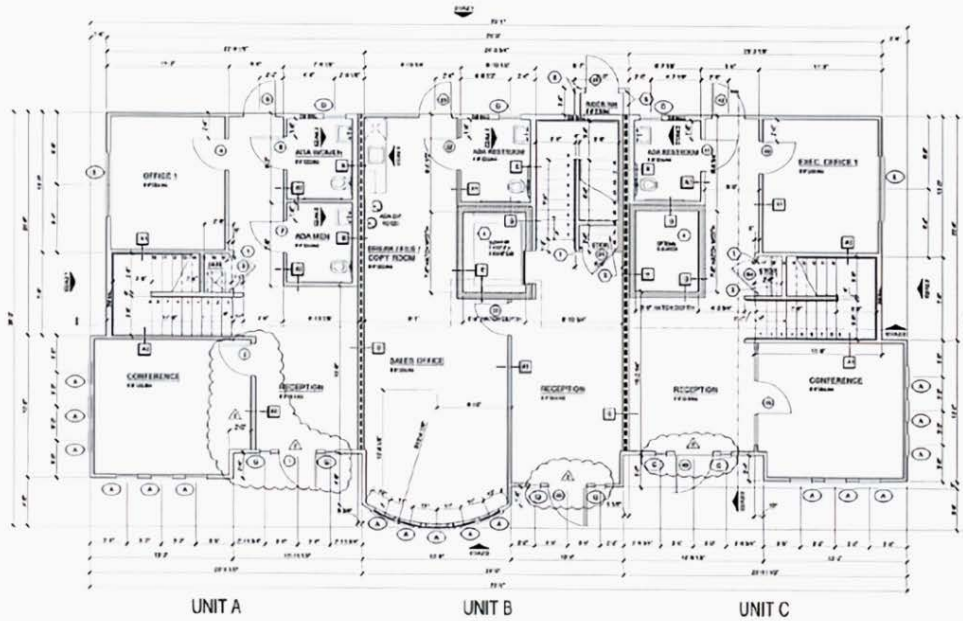
First Floor
