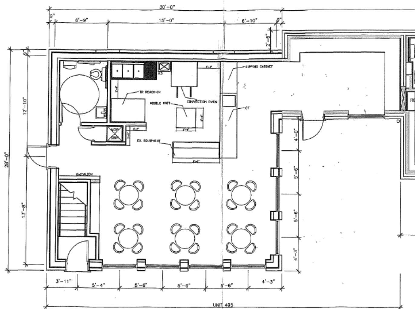
FIRST FLOOR PLAN SCALE: \frac{3}{16}" = 1'-0"
