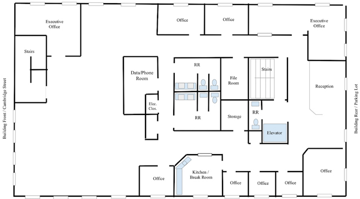
281 CAMBRIDGE STREET, BURLINGTON, MA 2 nd FLOOR
