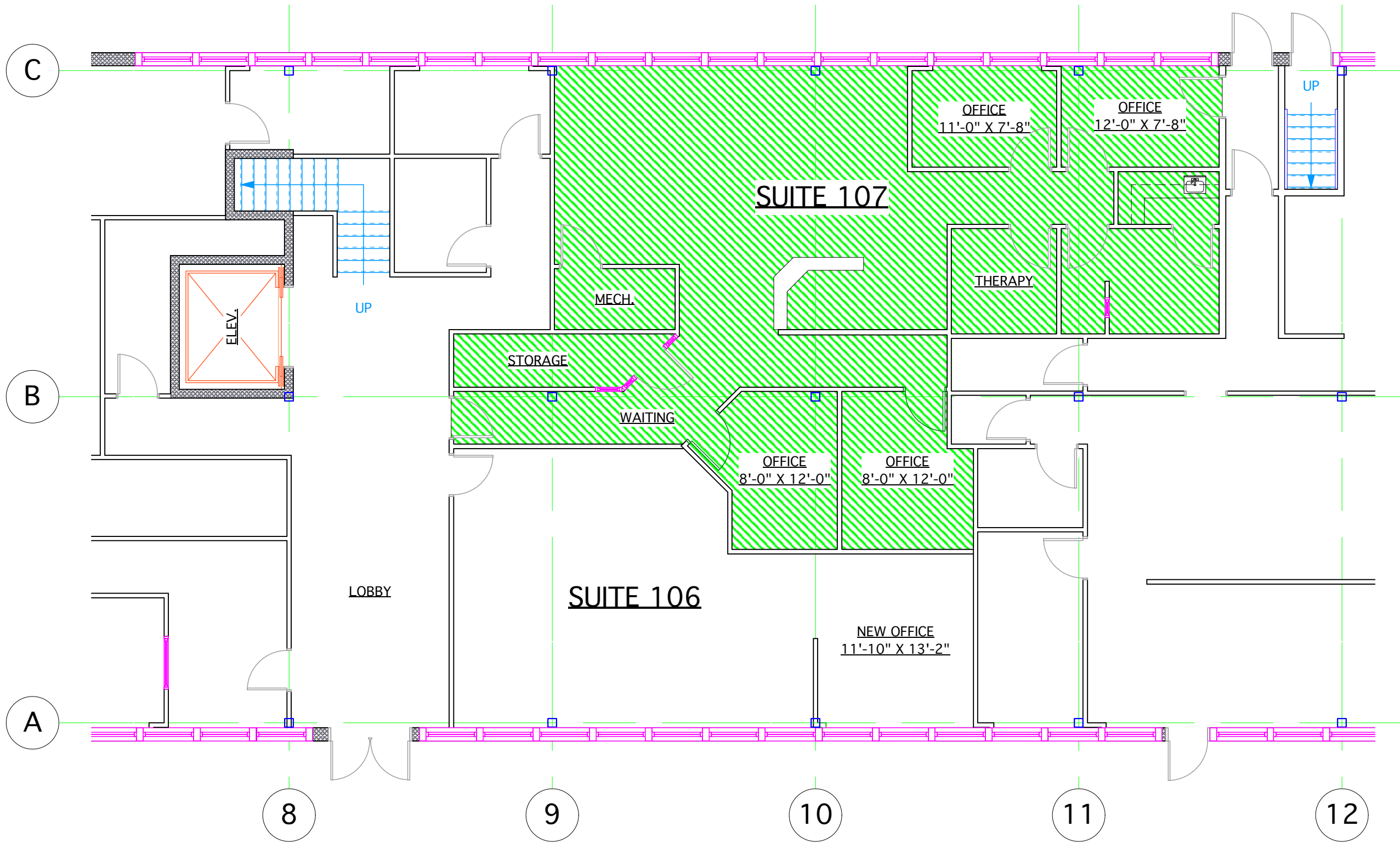
1 PARTIAL FIRST FLOOR PLAN A-2 Scale: 1/8" = 1'-0" NOTE : ALL DIMENSIONS ARE TO BE VERIFIED IN THE FIELD.
