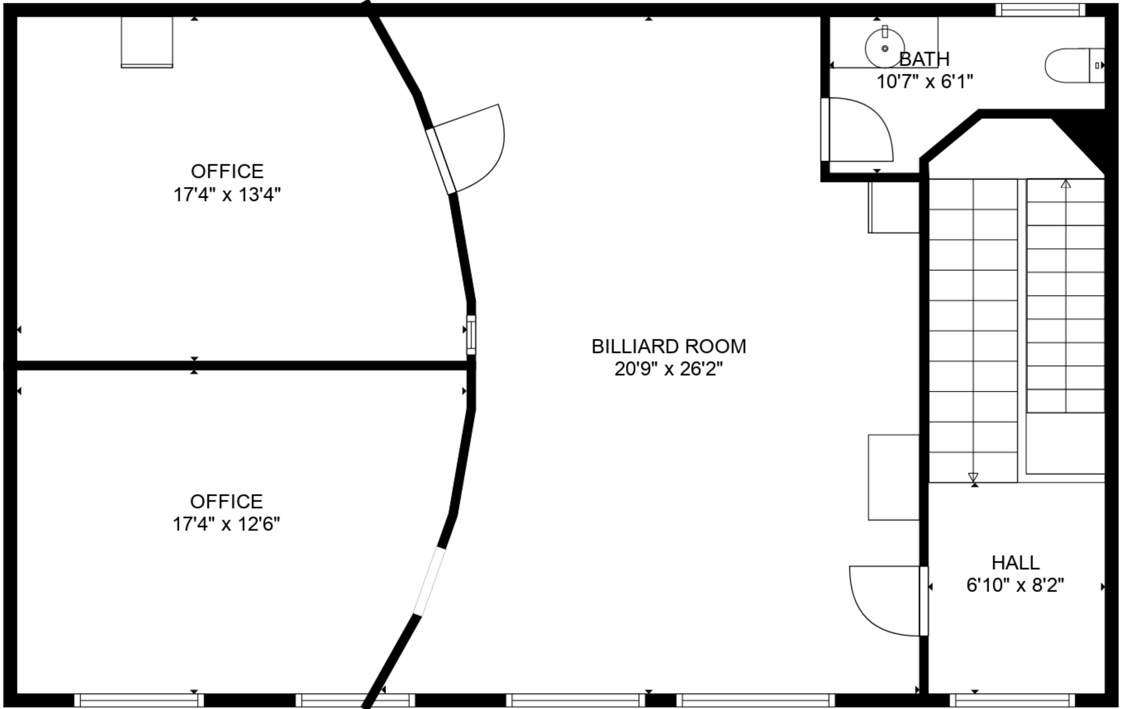
FLOOR 3
