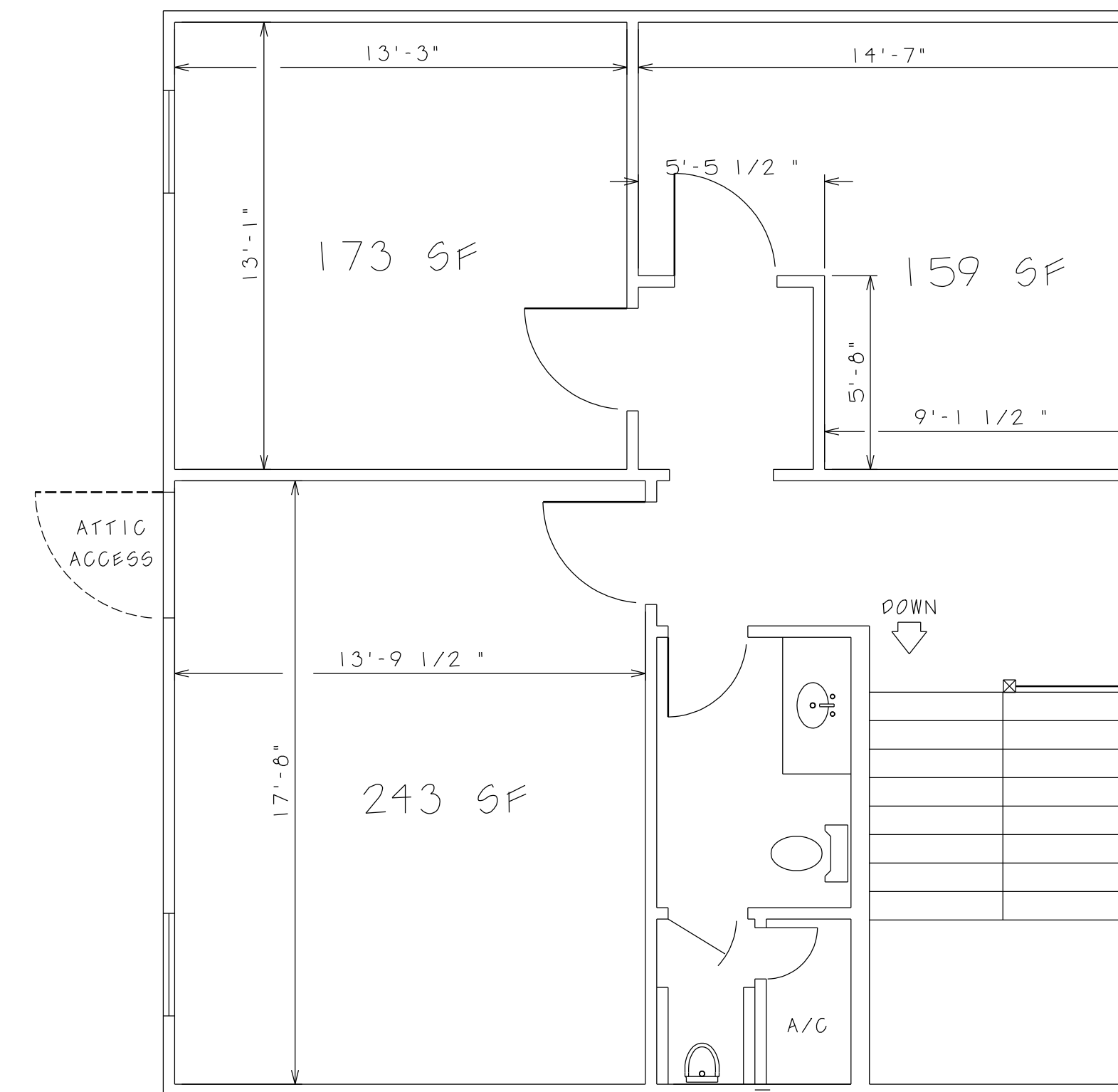
2ND FLOOR PLAN VIEW
