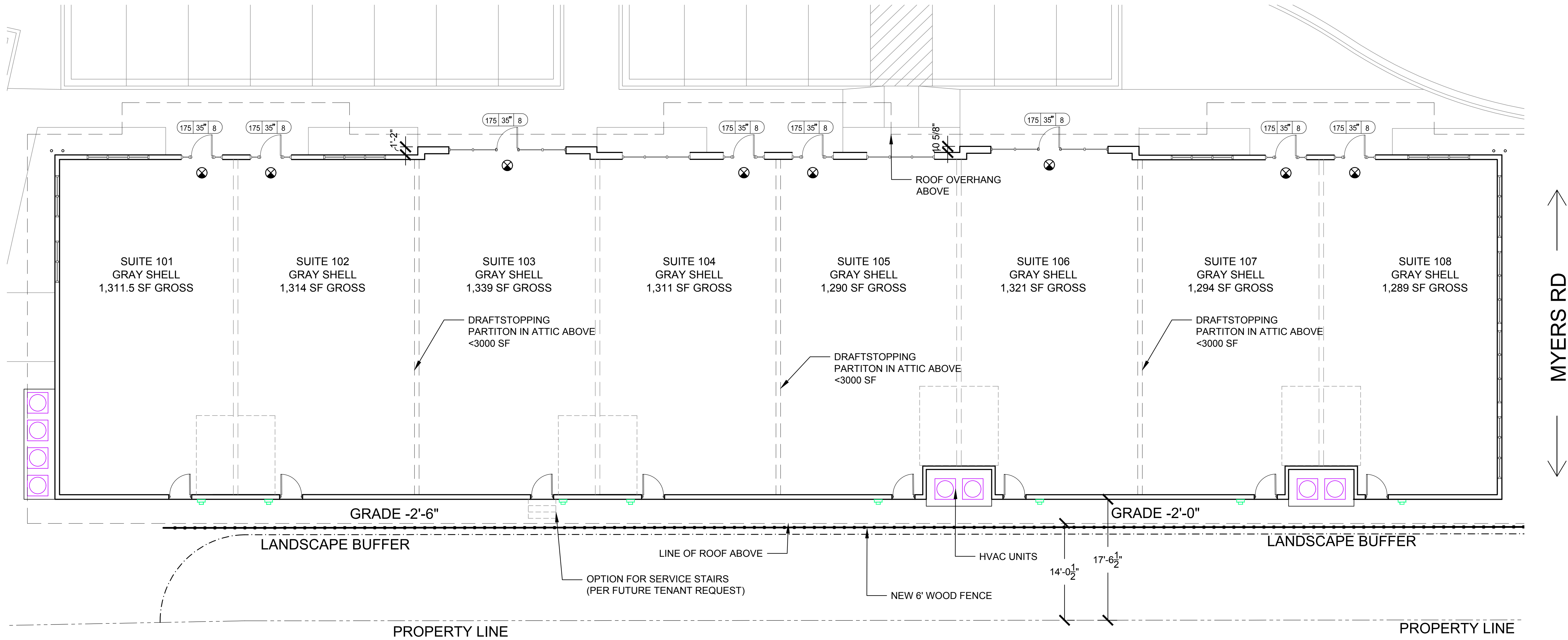
1 LIFESAFETY PLAN SCALE: 1/8"=1'-0"
