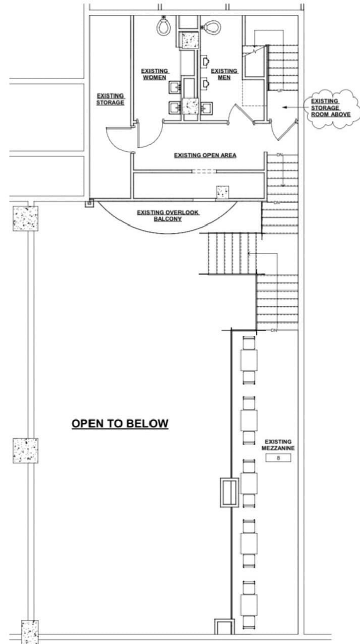
2 EXISTING 2ND FLOOR 1/4" = 1'-0"
