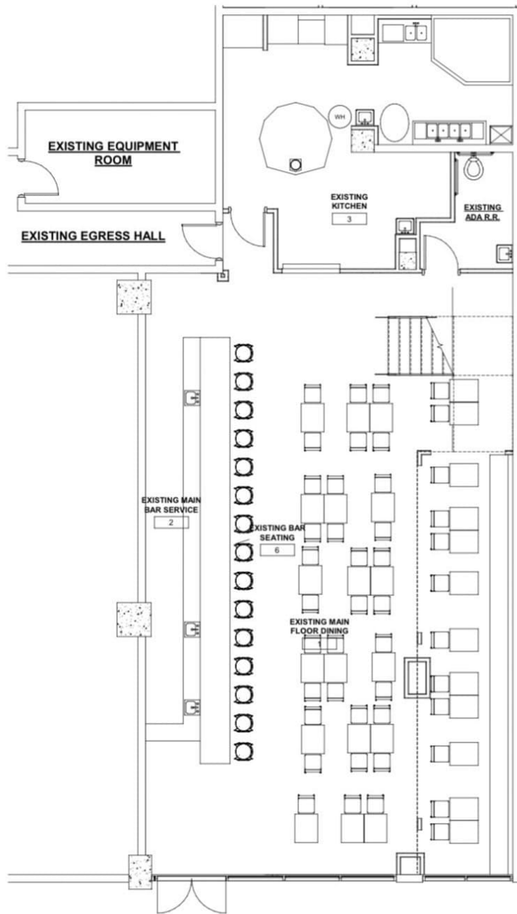
1 EXISTING MAIN FLOOR 1/4" = 1'-0"
