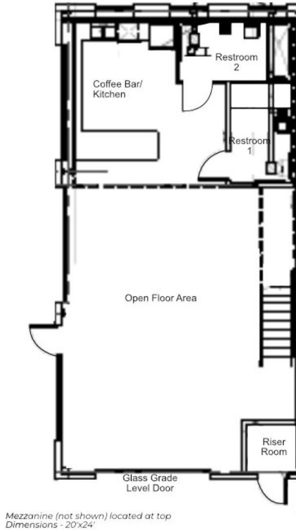
Clubhouse - Floor Plan
