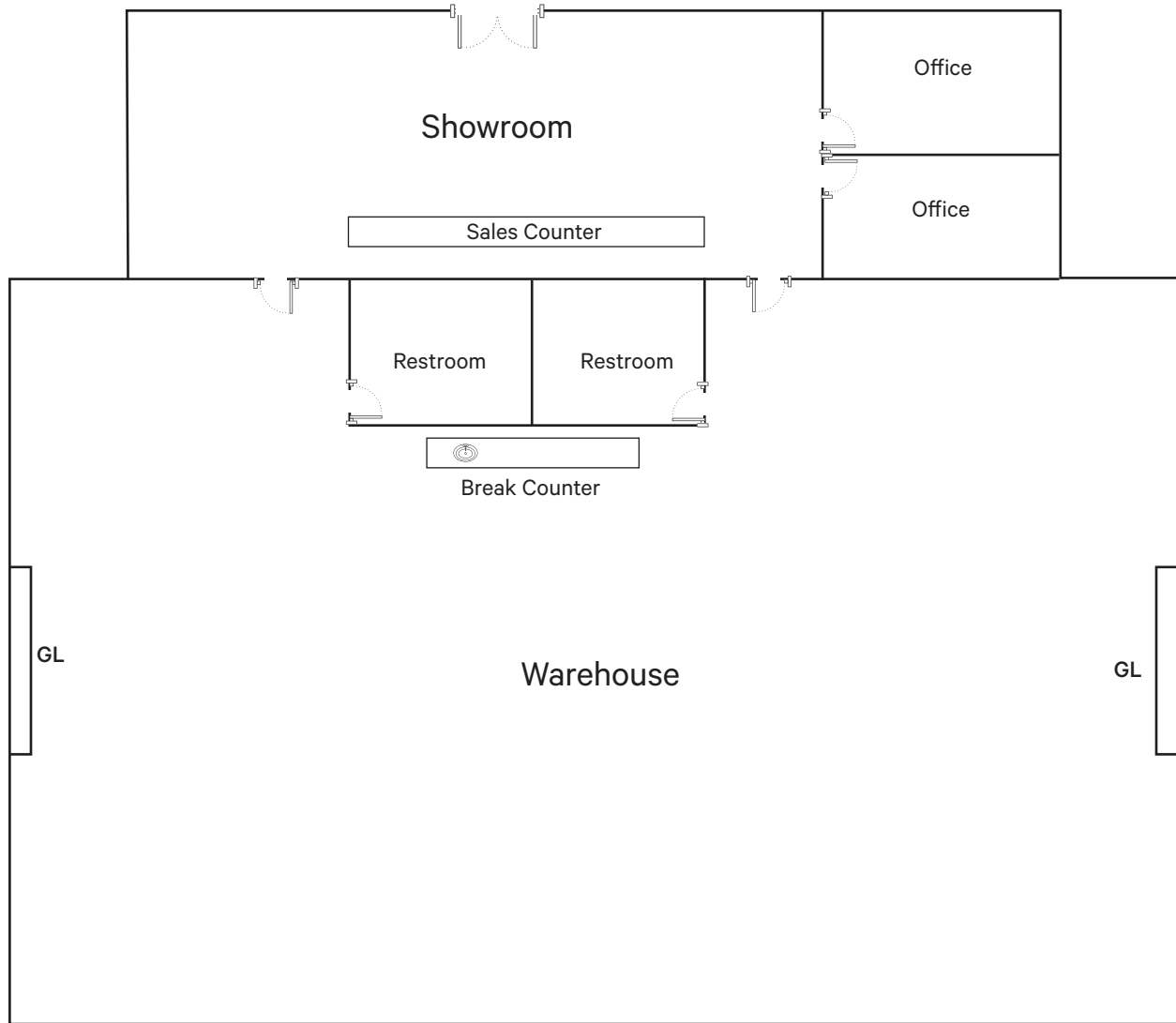
Floor plan not to scale GL = 14'x14' Grade Level Door
