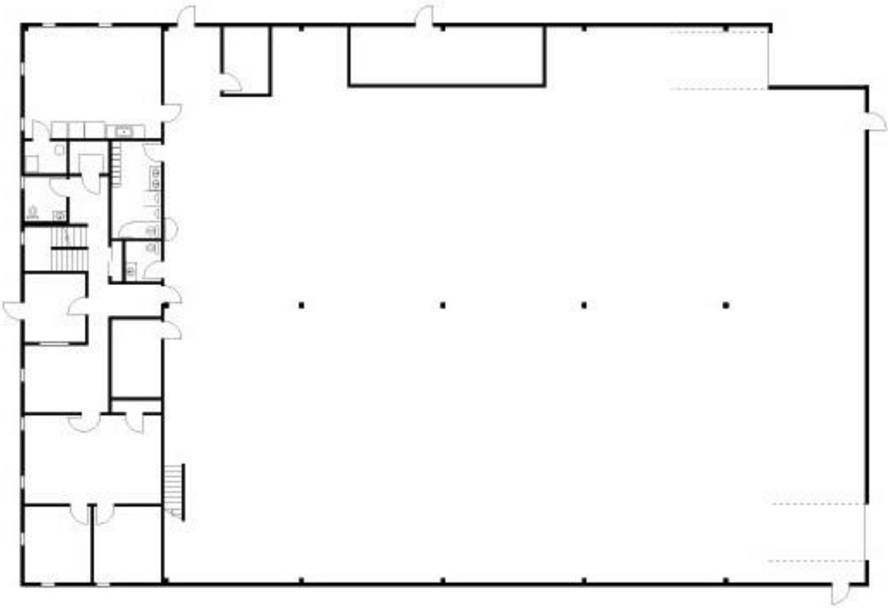
Warehouse/1 st floor layout
