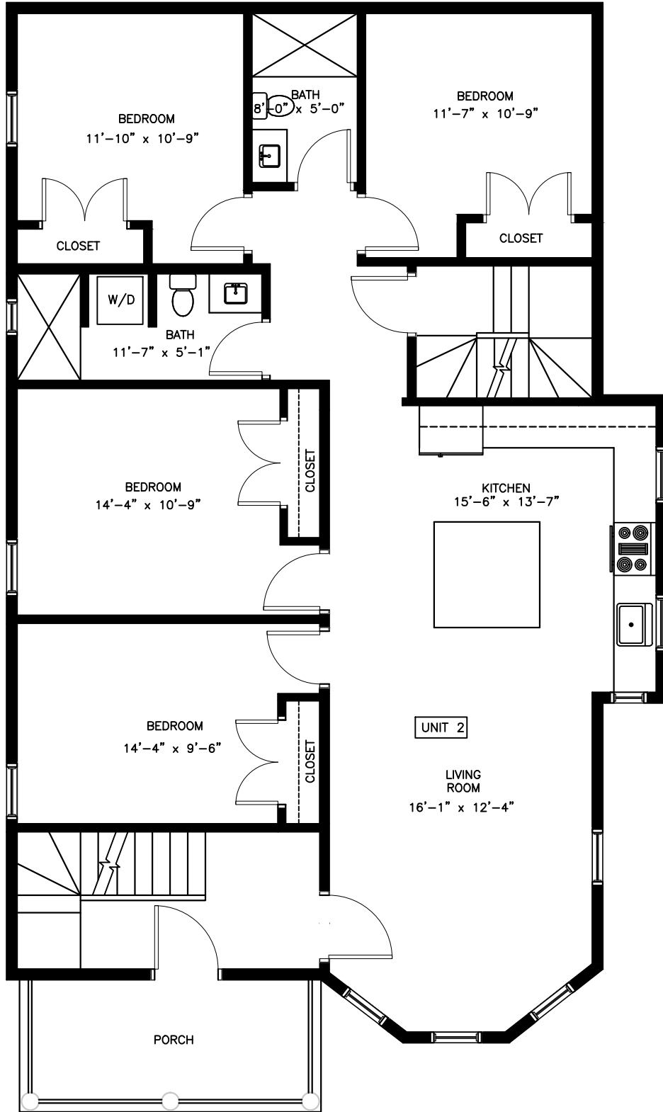
SECOND FLOOR PLAN UNIT 2
