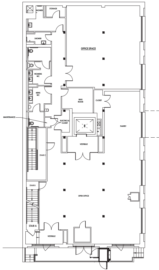
1 FIRST FLOOR PLAN SCALE: 3/16" = 1'-0"
