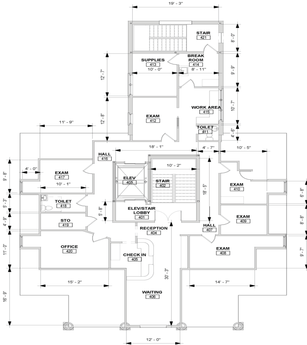
FOURTH FLOOR PLAN
