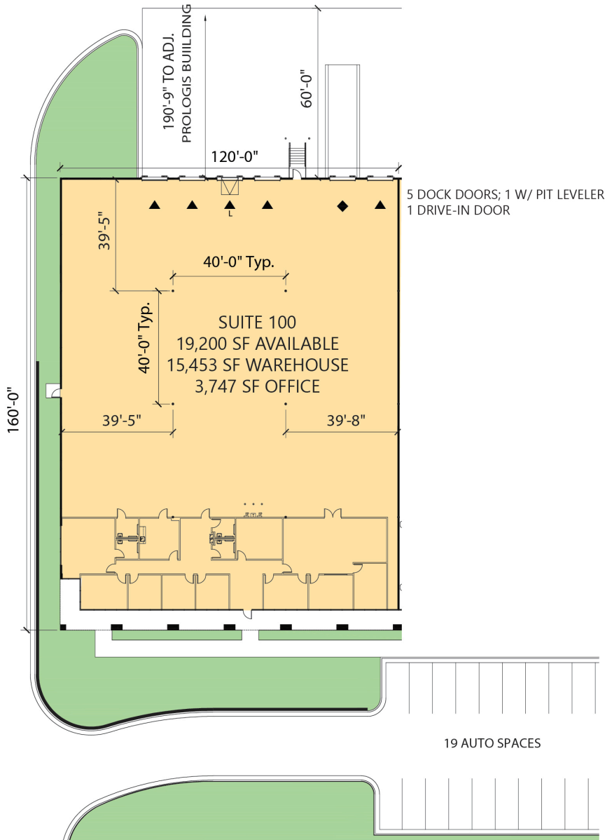
KEY PLAN
