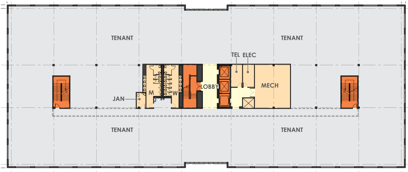
TYPICAL FLOORPLATE: 30,000+ SF
