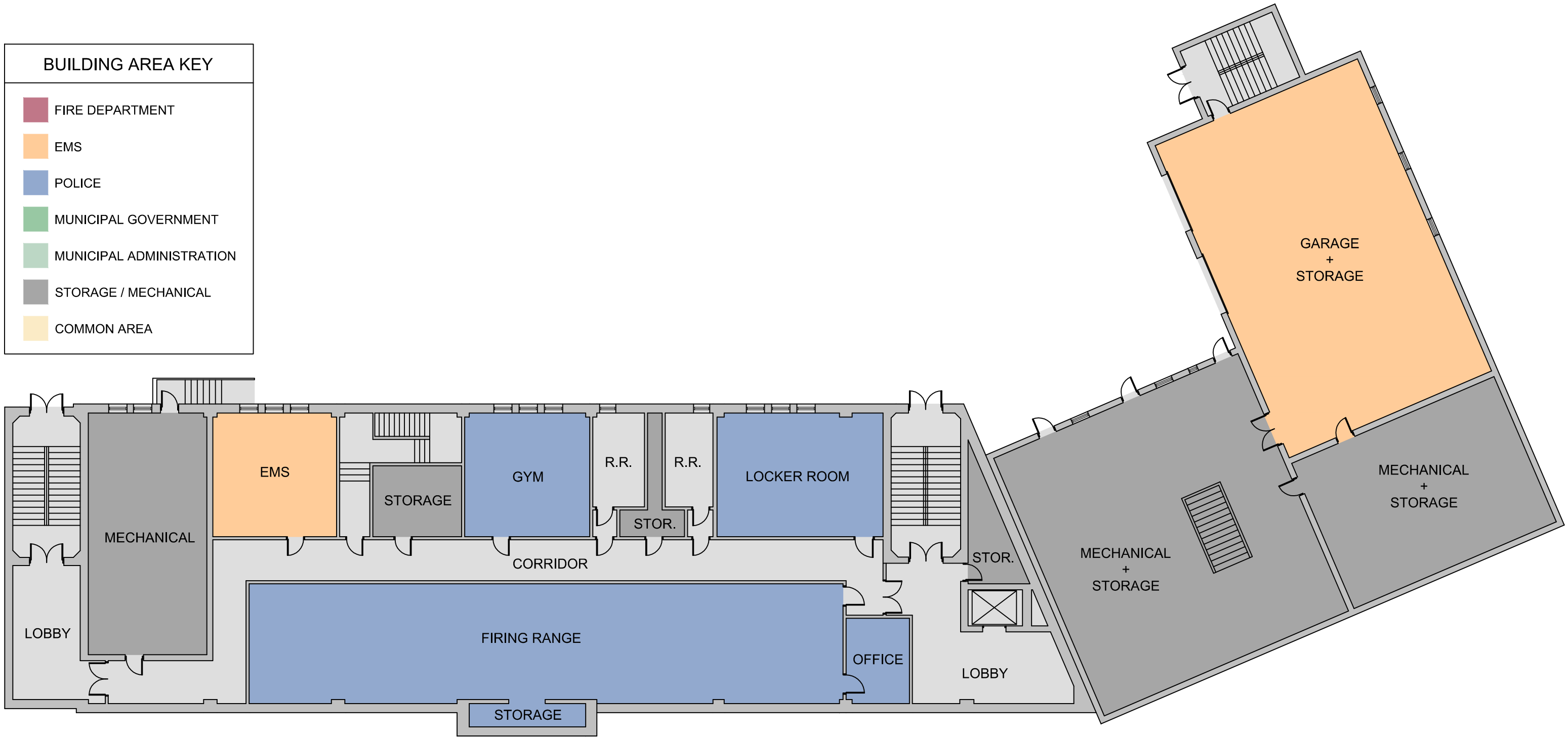
1 BASEMENT FLOOR PLAN SCALE: 1/16"=1'-0"
