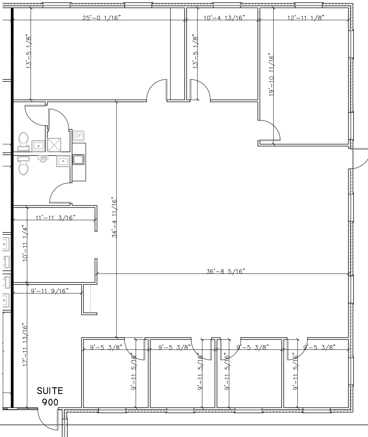
FLOORPLAN SCALE: 1/8" = 1'-0" (LETTER SIZE)
