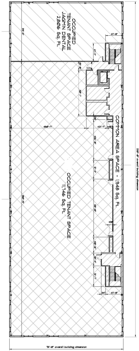
2 FLOOR PLAN SCALE: 3/32" = 1'-0" UPPER LEVEL LAYOUT
