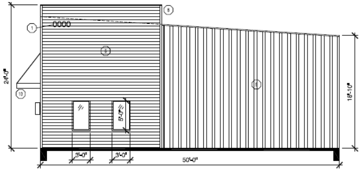
BLDG 1 - NORTH ELEVATION
