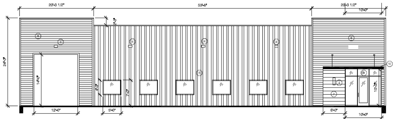
BLDG 1 - WEST ELEVATION
