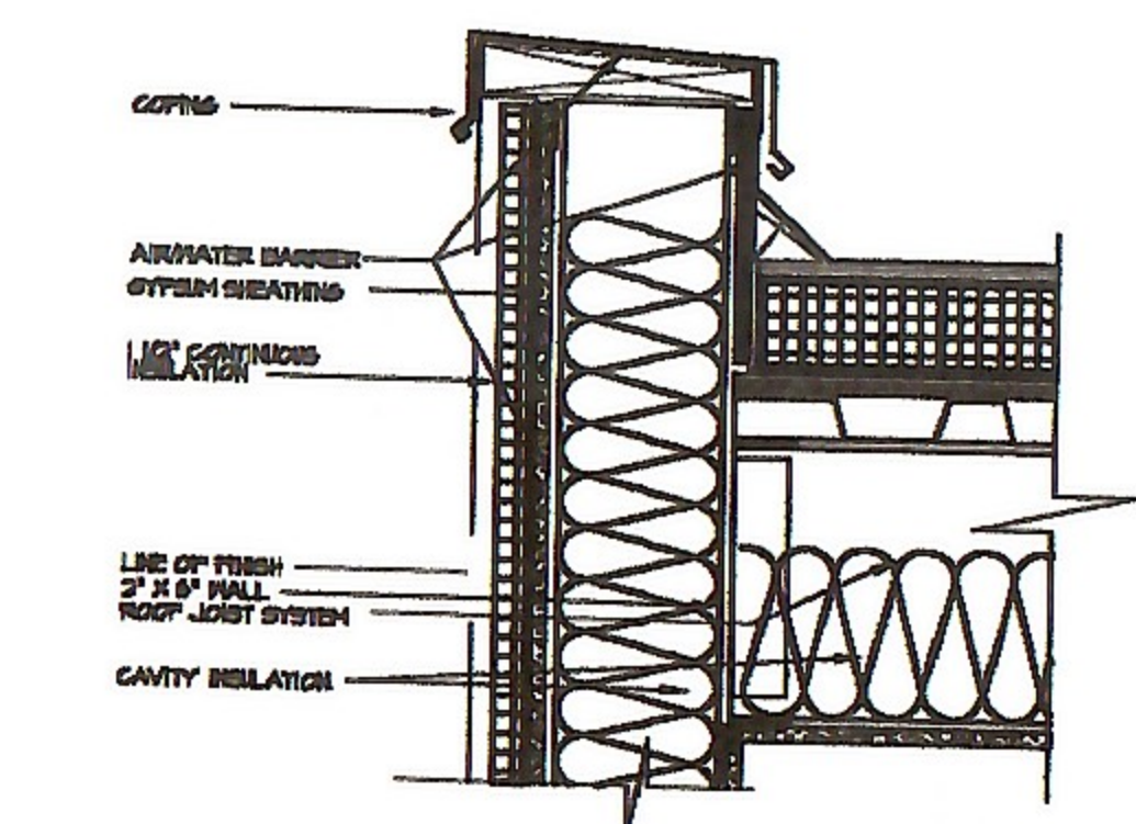
EIFS WALL SECTION SCALENTS
