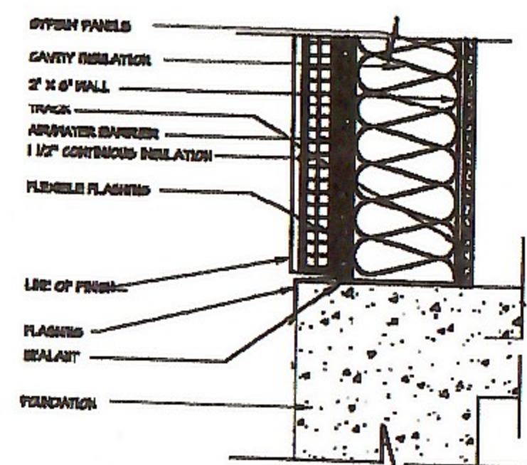
EIFS WALL SECTION SCALE: 1/8" = 1'-0"
