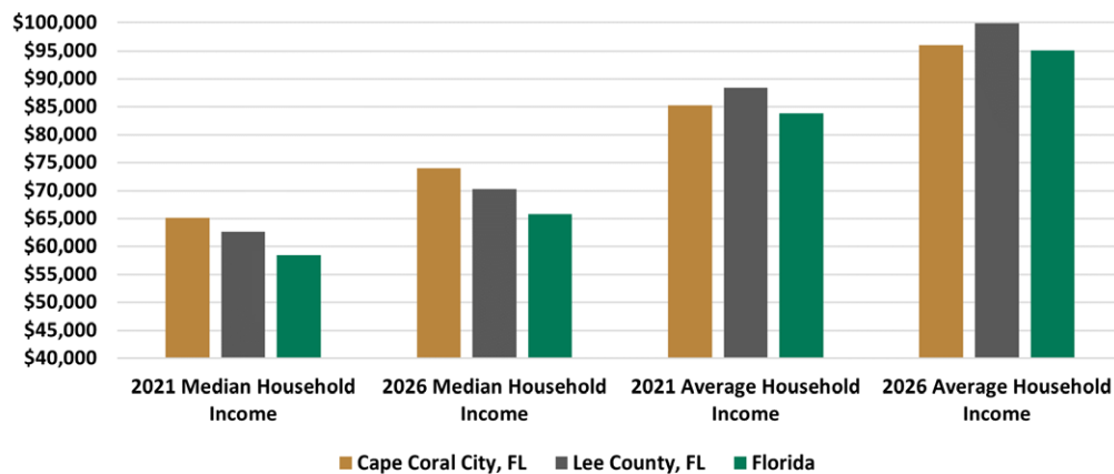
Household Incomes
