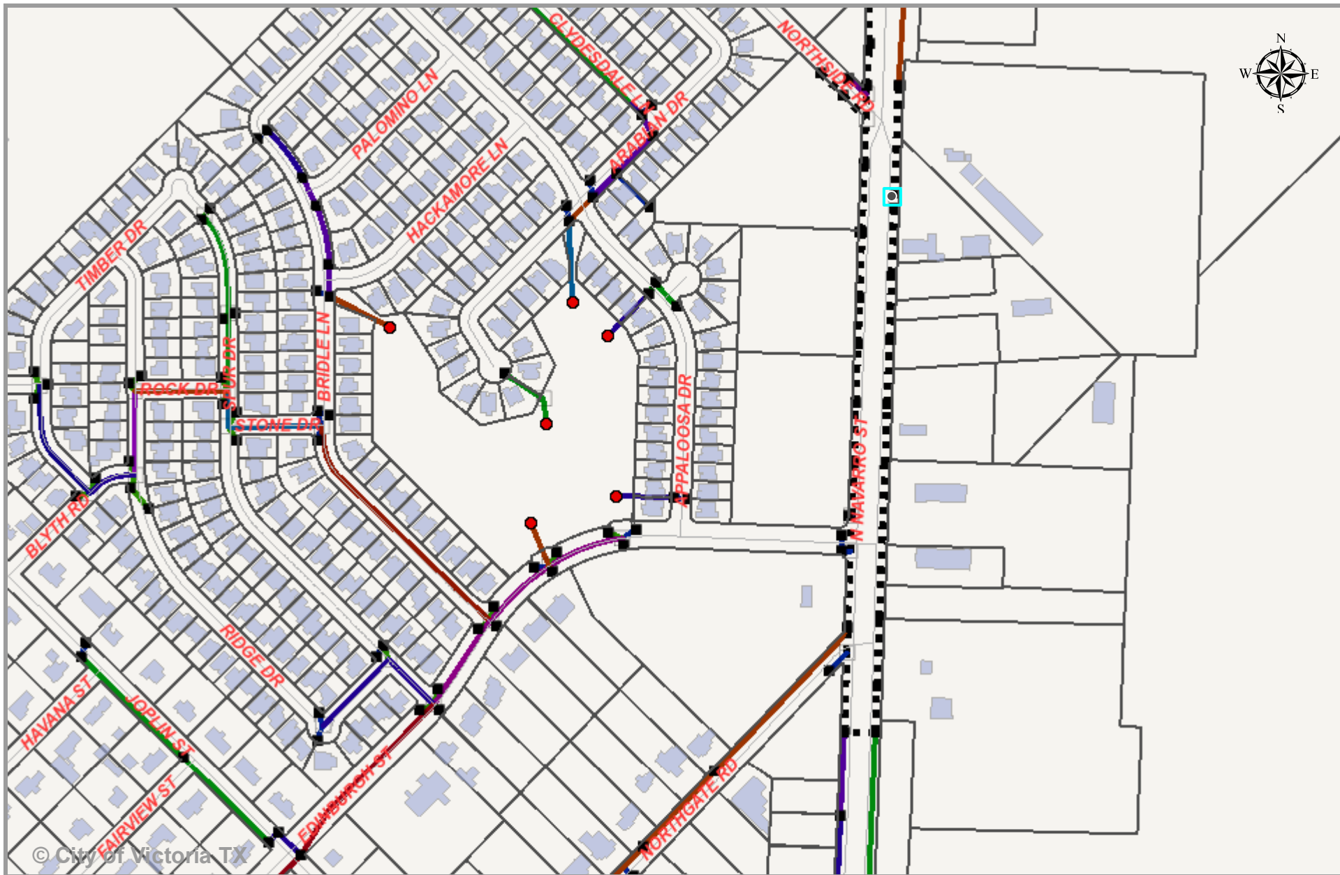
13002 N Navarro -Storm Sewer Map
