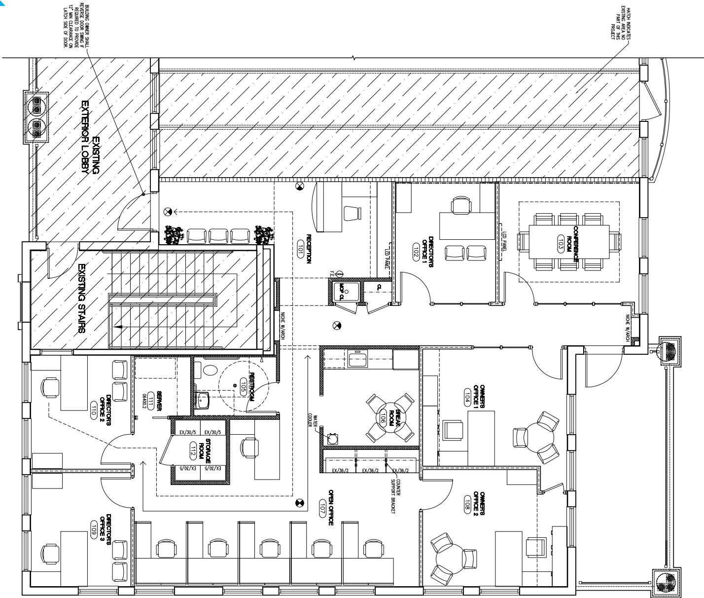
EQUIPMENT PLAN AND LIFE SAFETY DIAGRAM
