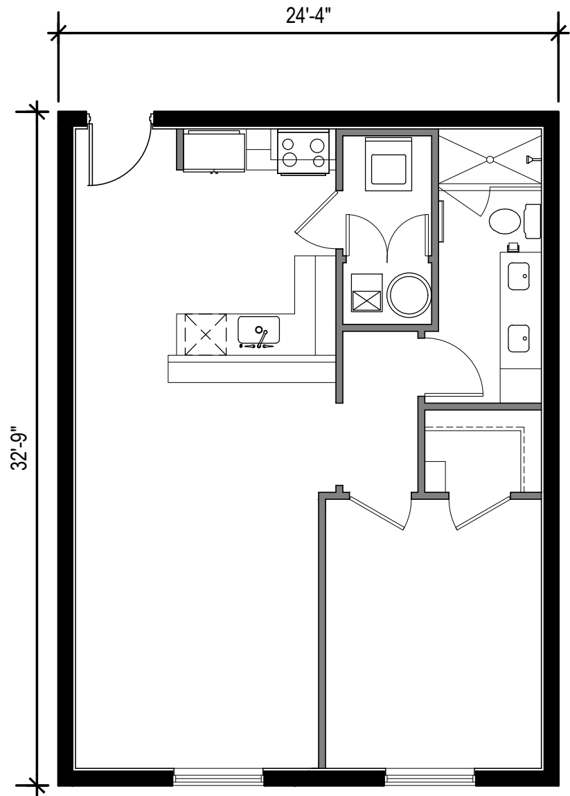
UNIT "A1" FLOOR PLAN
