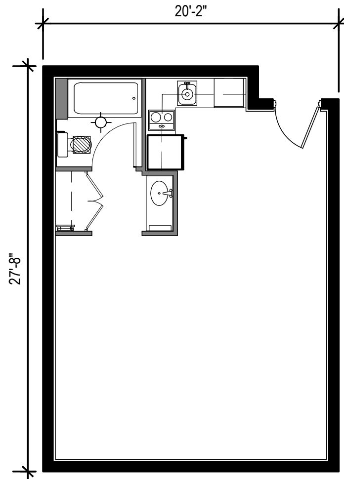
UNIT "S2" FLOOR PLAN
