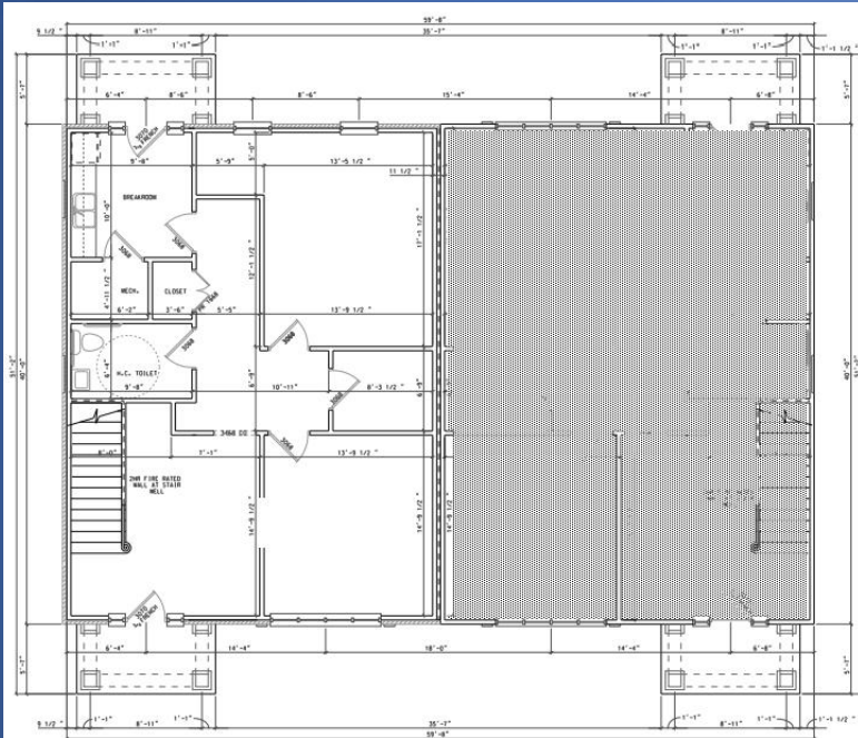
floor plan - two story
