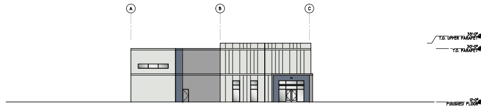
NORTH ELEVATION (DOCKS)
