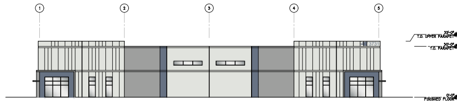
WEST ELEVATION (BOMBARDIER COURT)
