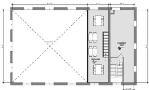
3 MEZZANINE & THIRD FLOOR PLAN UP + 2.0'
