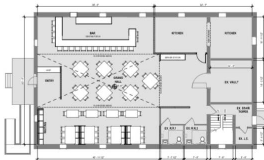
1 FIRST FLOOR PLAN UP + 2.0'
