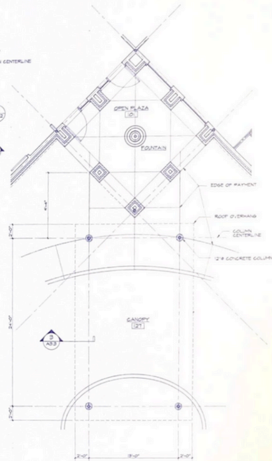
DRIVE-THRU CANOPY PLAN
