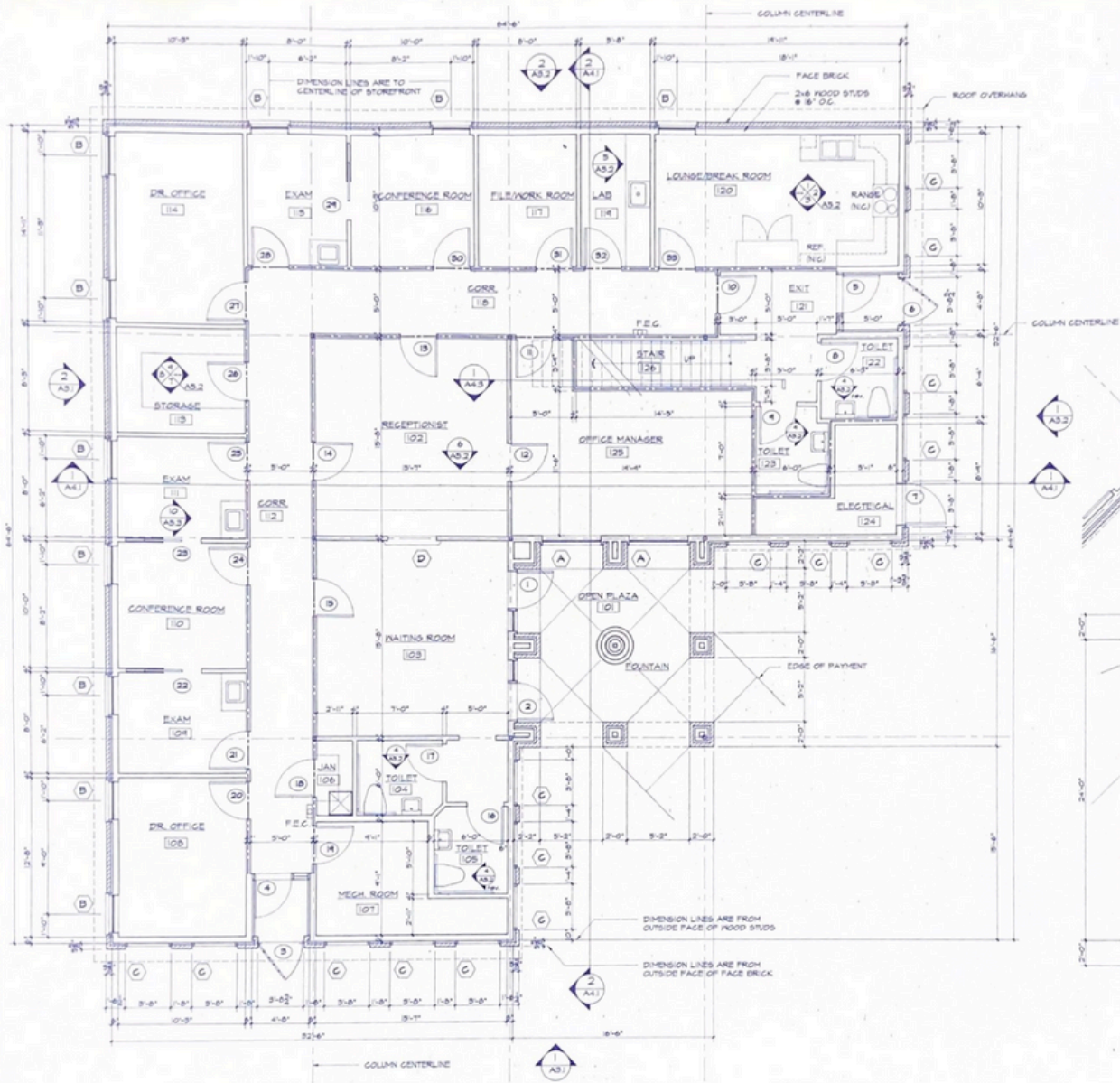
ENTRY LEVEL FLOOR PLAN
