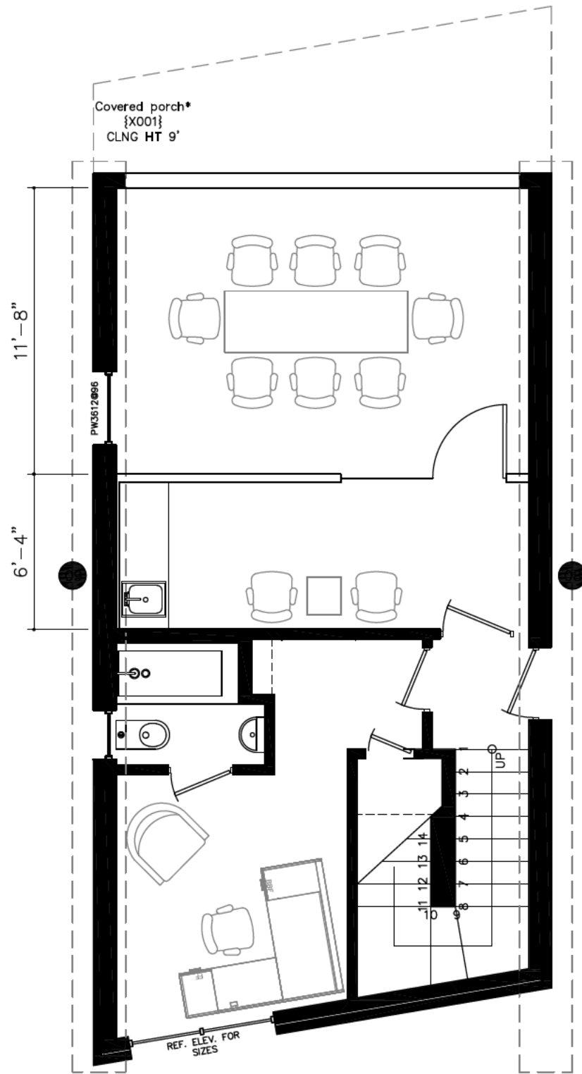
LEVEL 1 PLAN
