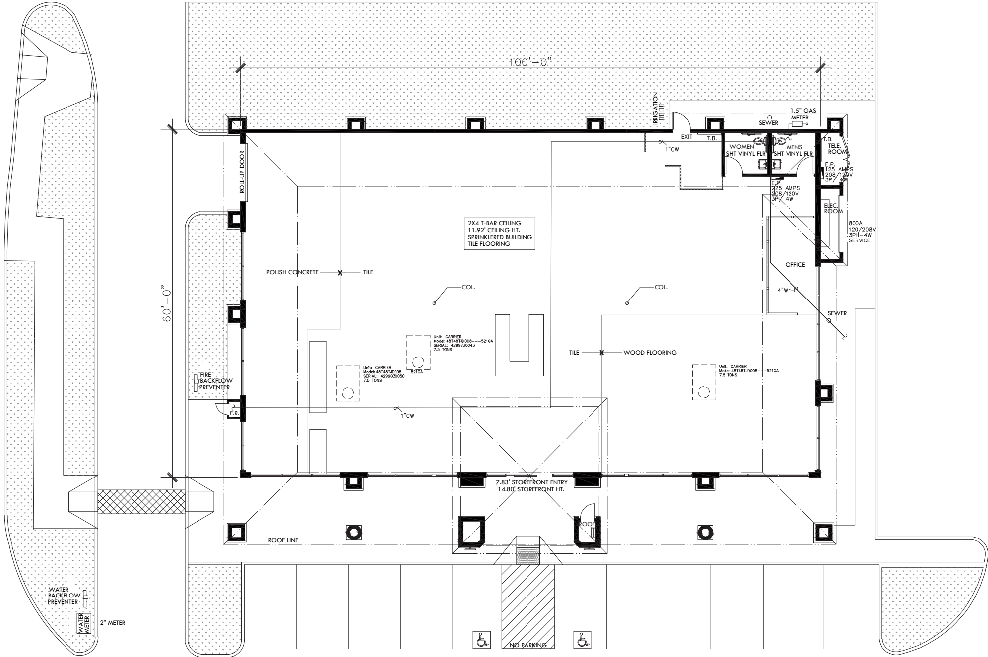
AS-BUILT FLOOR PLAN APPROX. 6,000± S.F.
