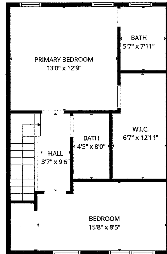
3rd floor
