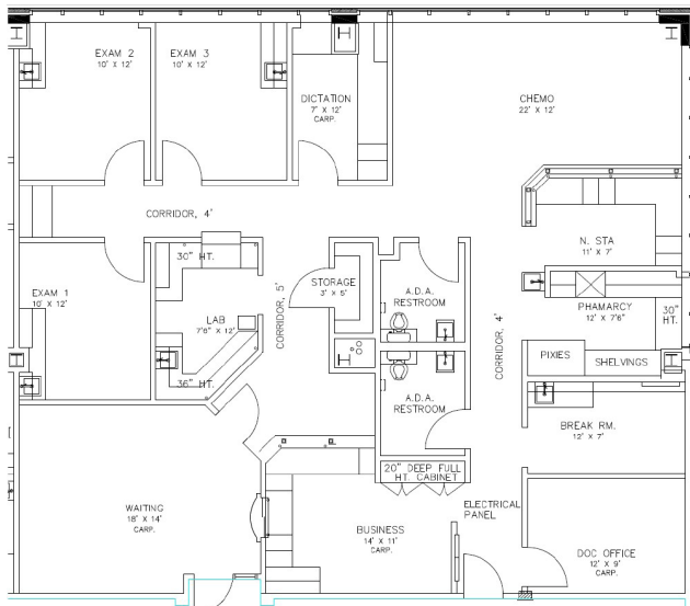
CONCEPTUAL LAYOUT
