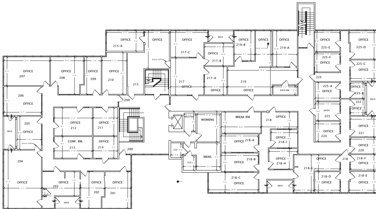
1 EXISTING SECOND LEVEL FLOOR PLAN 12,165 SQFT GROSS MEASURED AREA 350 SQFT MEASURED EXTERIOR SURFACES
