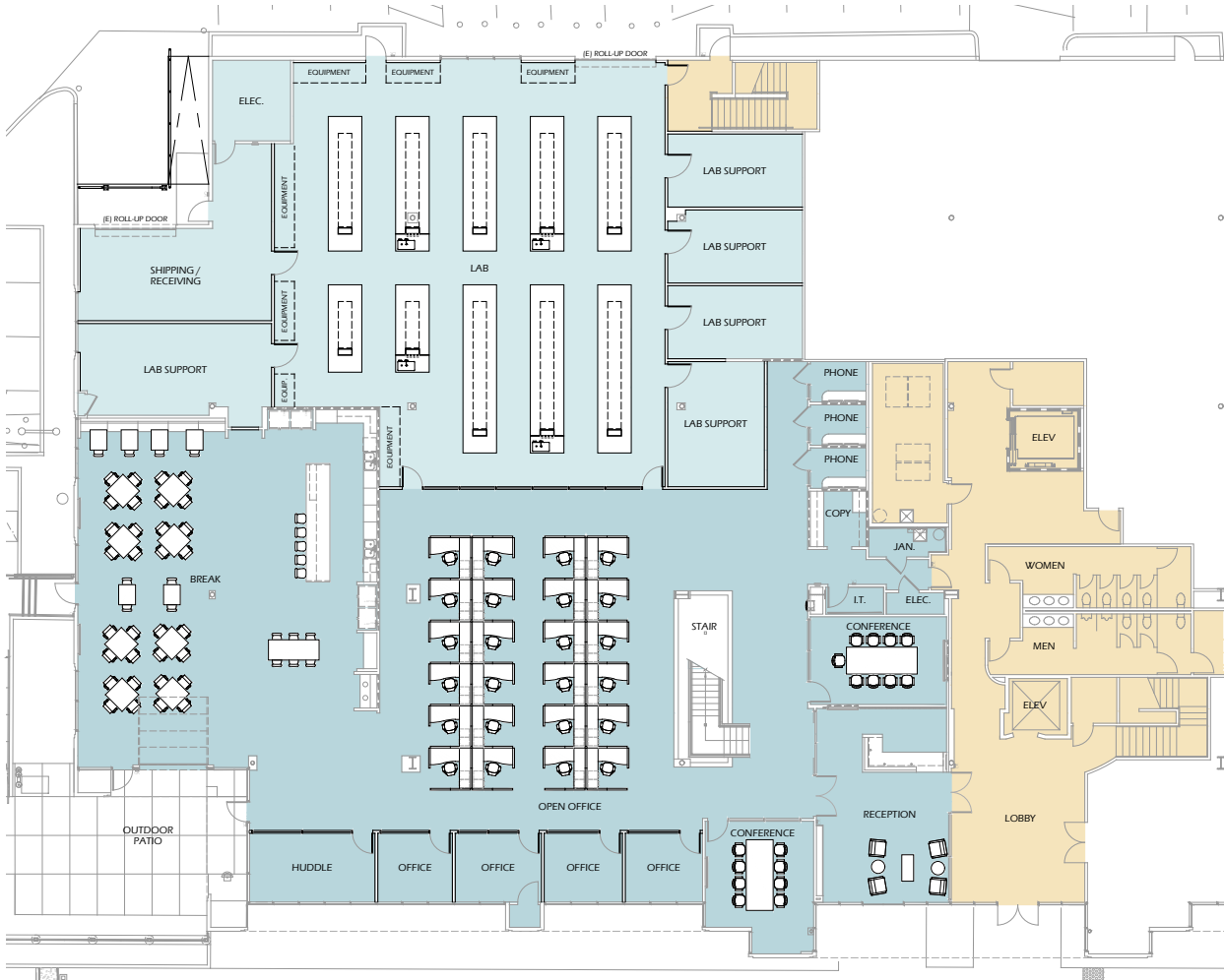
CONCEPTUAL PLAN
