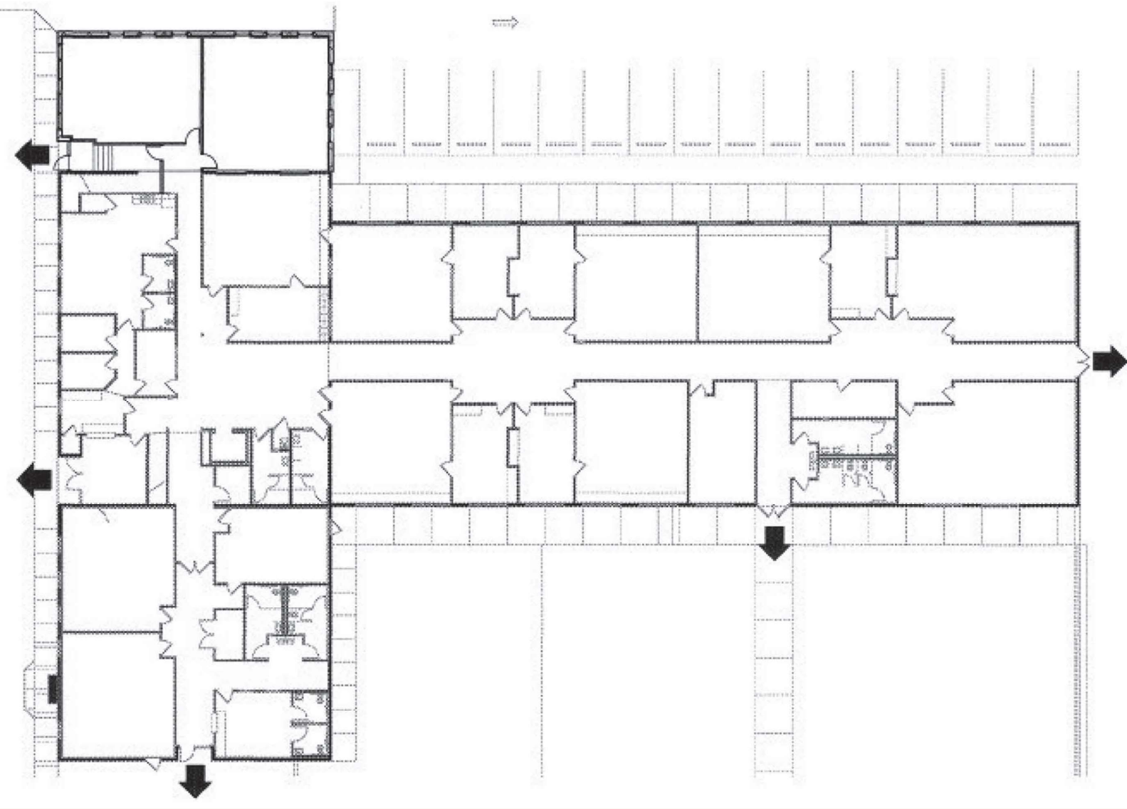
1st Floor
