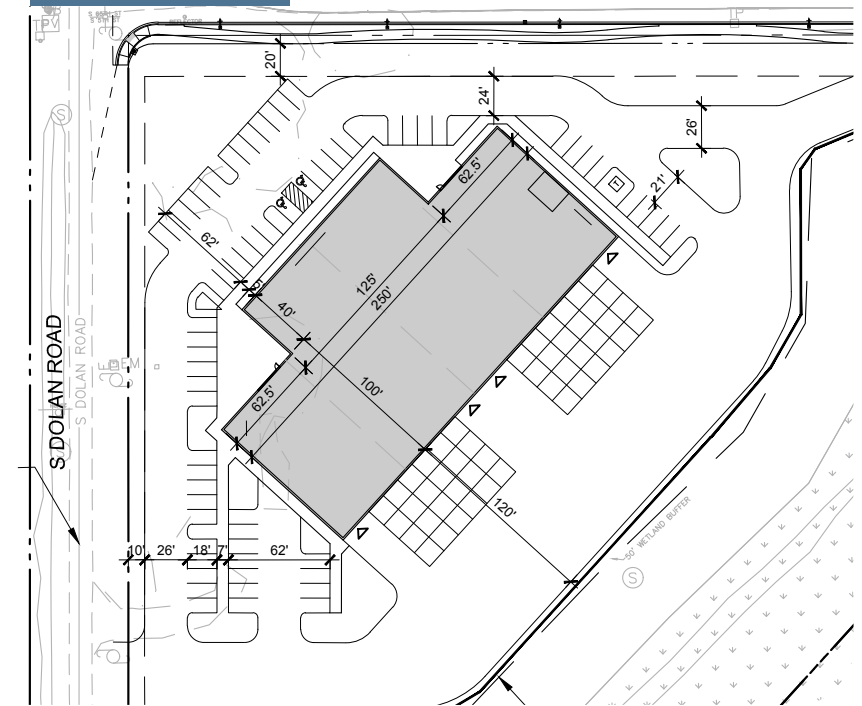
Conceptual Site Plan 2*
