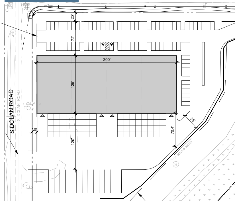
Conceptual Site Plan 1*
