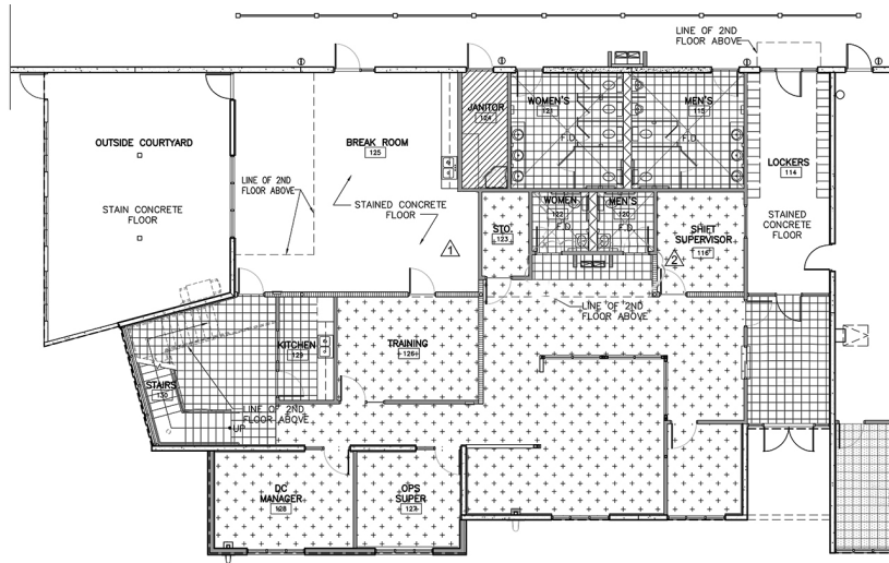
1ST FLOOR - MAIN OFFICE (±5,843 SF)
