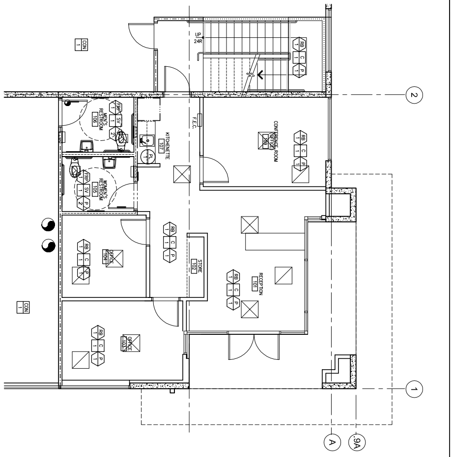
ENLARGED 1ST FLOOR FINISH PLAN SCALE: 1/4"=1'-0"
