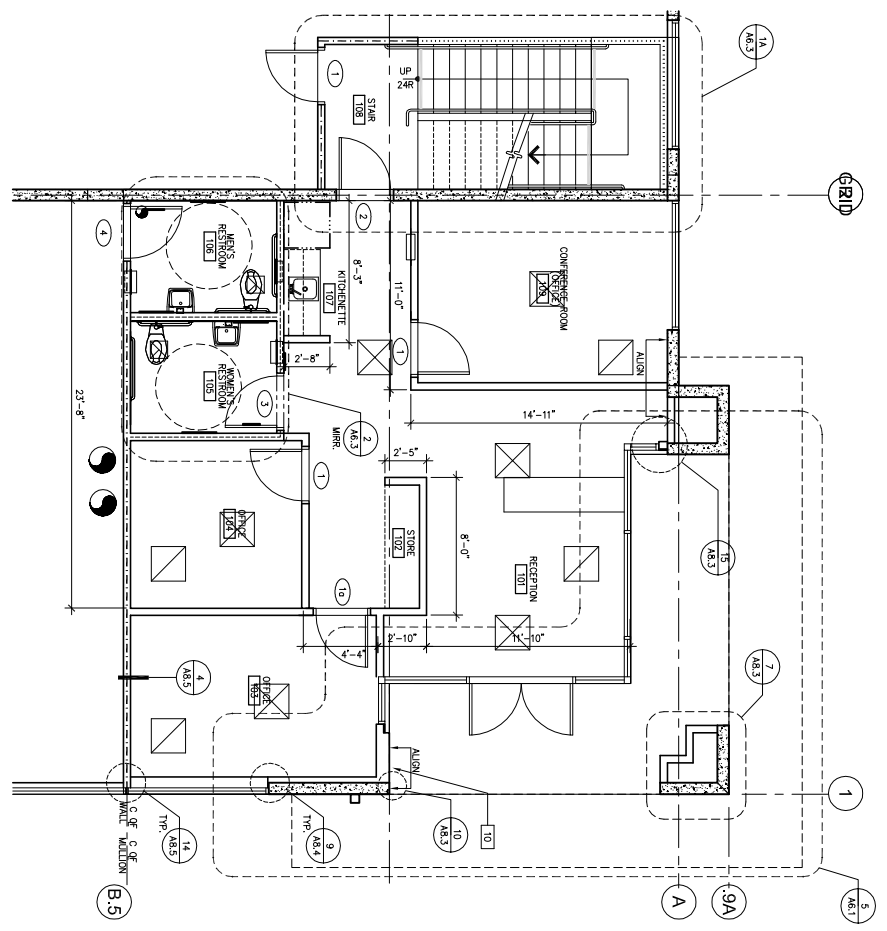
ENLARGED 1ST FLOOR PLAN SCALE: 1/4"=1'-0"
