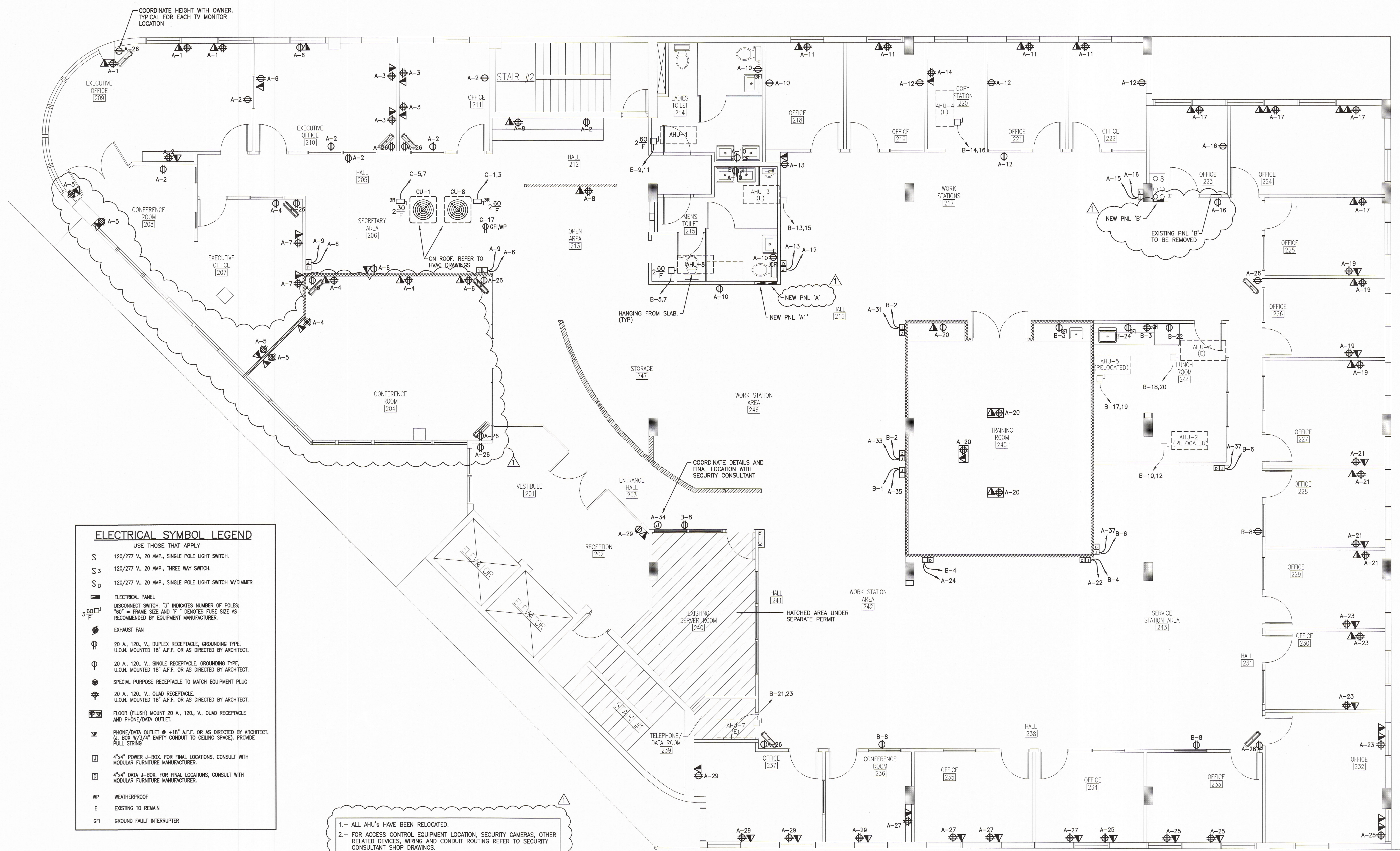
Power Plan 2nd Floor Scale: 3/16" = 1'-0" N
