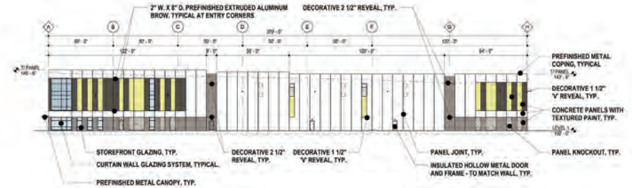
WEST ELEVATION
