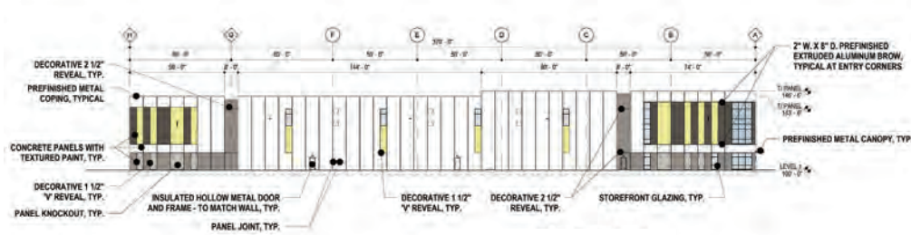
EAST ELEVATION
