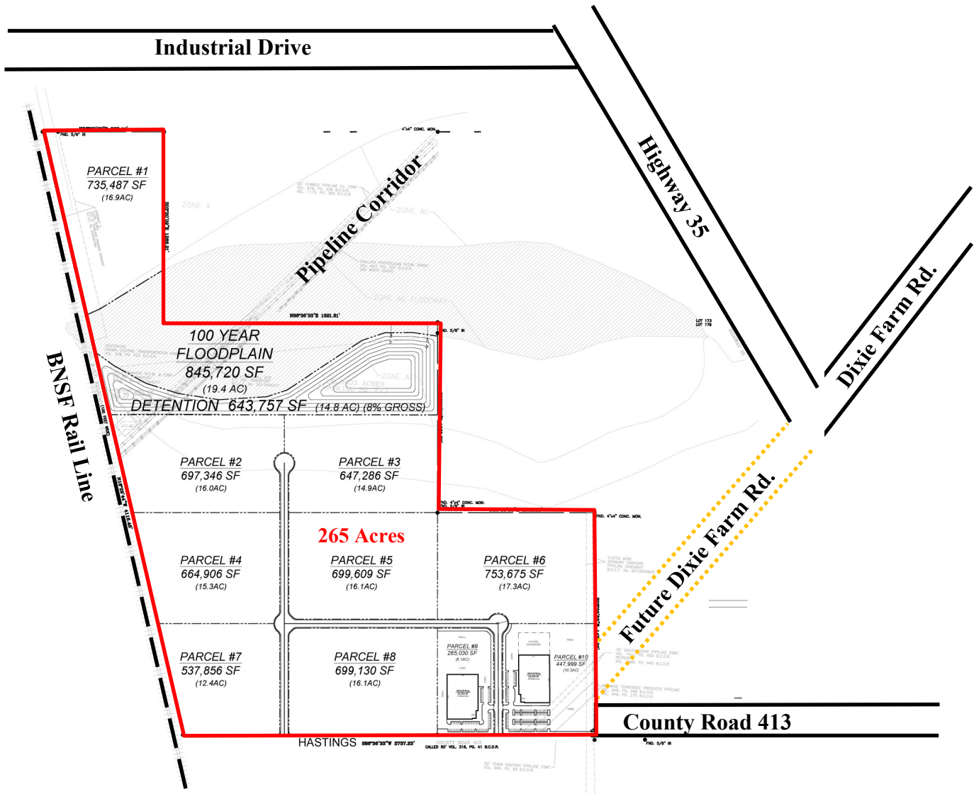
Conceptual Industrial Park Layout
