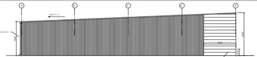
South Elevation
