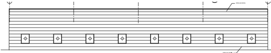
East Elevation
