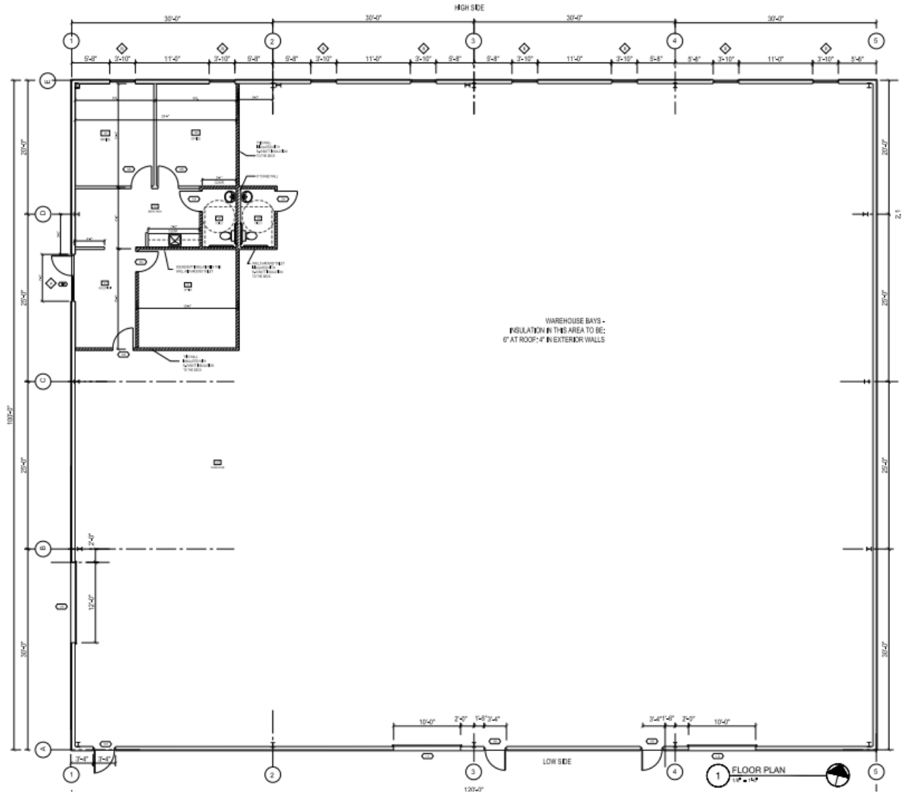
Floor Plan
