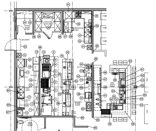
01 floor plan 1/8" = 1'-0"
