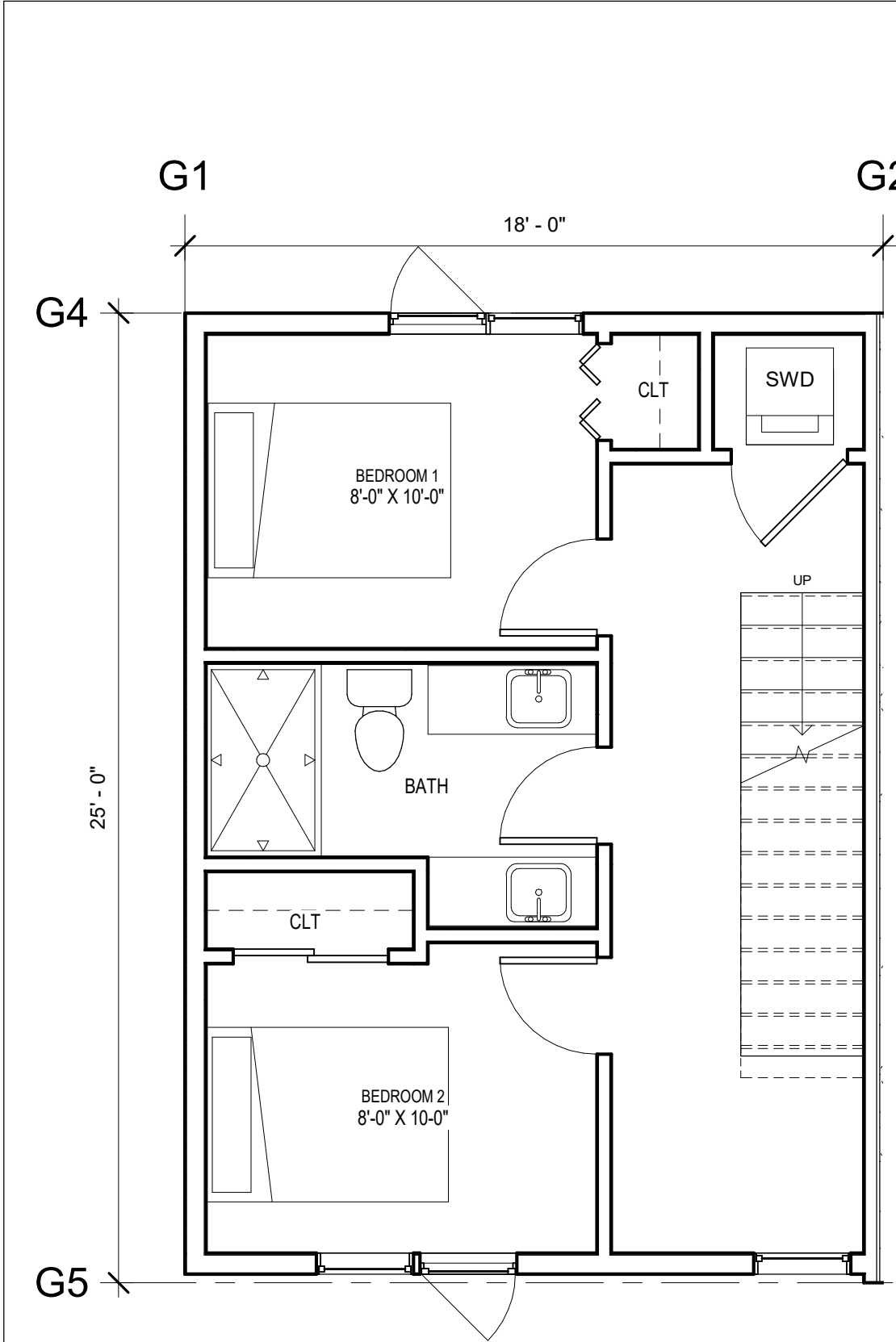
① UNIT 1 L2 1/4" = 1'-0"
