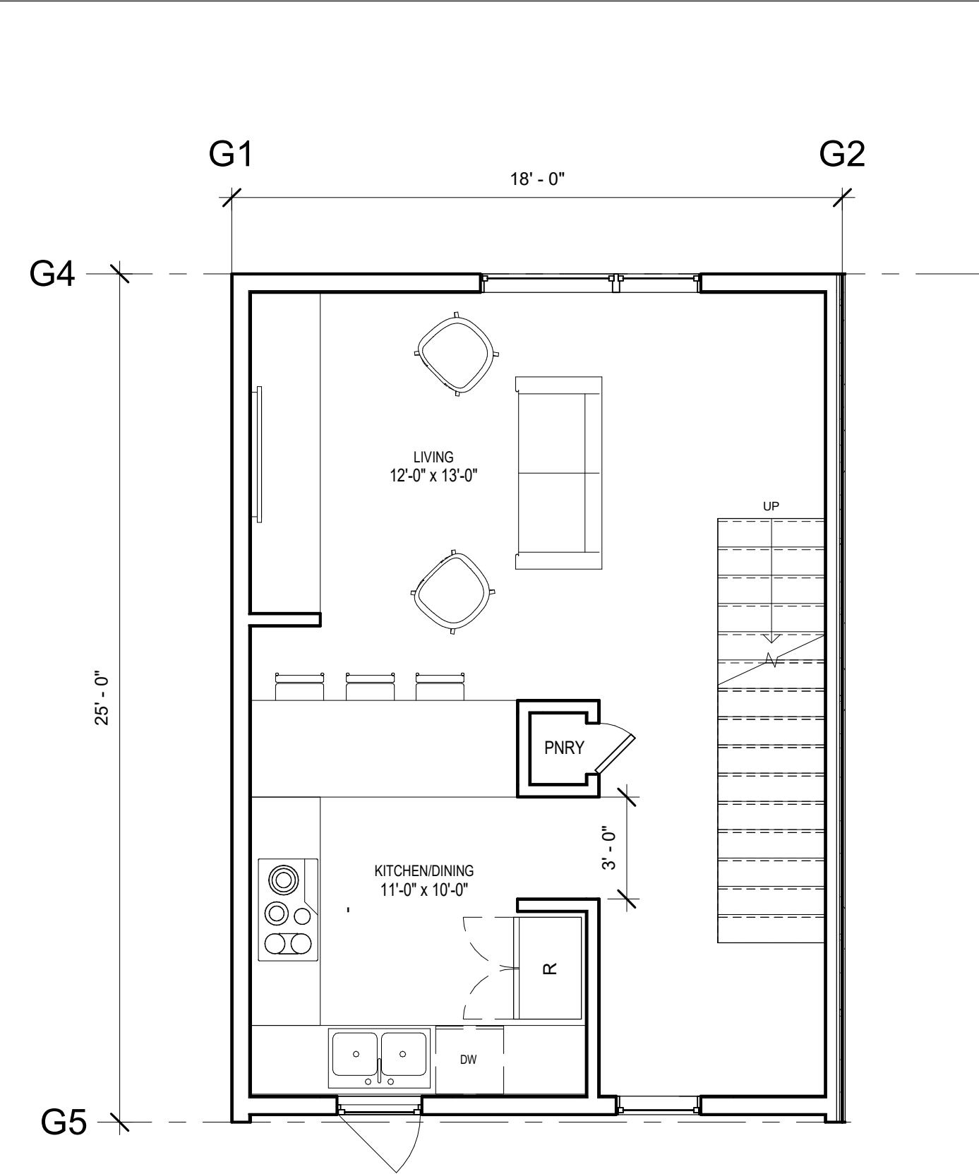
② UNIT 1 L3 1/4" = 1'-0"
